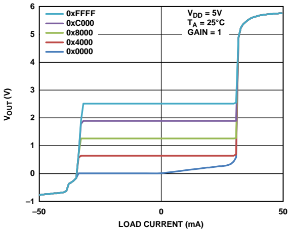
Figure 34. Source and Sink Capability, Gain = 1
