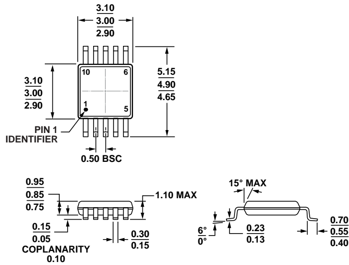
Figure 53. 10-Lead Mini Small Outline Package [MSOP] (RM-10) Dimensions shown in millimeters
