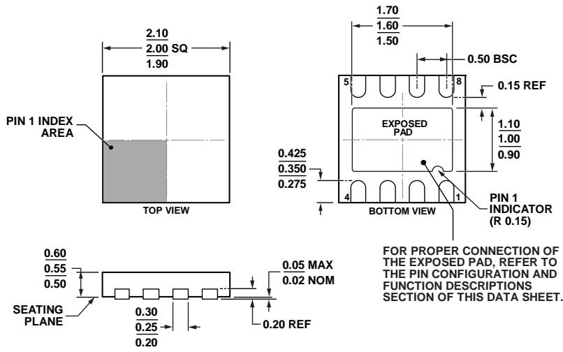
Figure 52. 8-Lead Lead Frame Chip Scale Package [LFCSF_UD] 2.00 mm × 2.00 mm Body, Ultra Thin, Dual Lead (CP-8-10) Dimensions shown in millimeters
