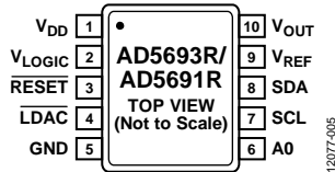
Figure 5. AD5693R/AD5691R Pin Configuration, 10-Lead MSOP
