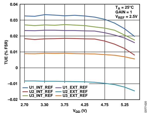
Figure 20. TUE vs. V_{DD}
