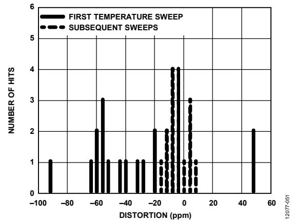
Figure 50. Thermal Hysteresis
