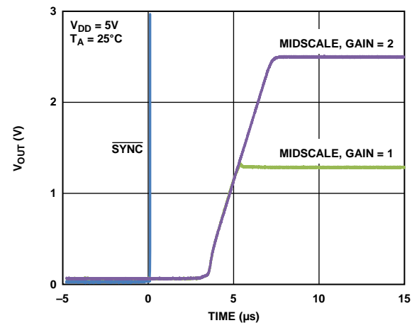
Figure 44. Exiting Power-Down to Midscale
