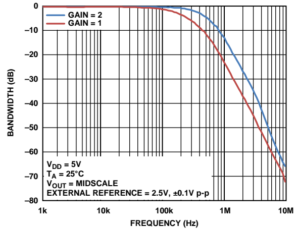
Figure 43. Multiplying Bandwidth, External Reference = 2.5 V, ± 0.1 V p-p, 10 kHz to 10 MHz
