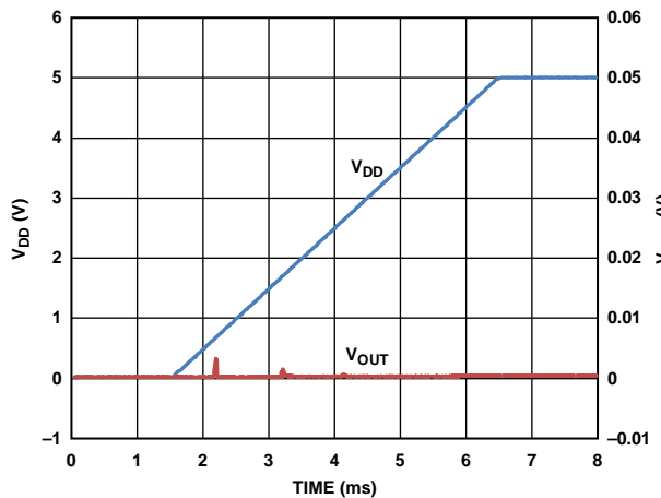
Figure 41. Power-On Reset to 0V
