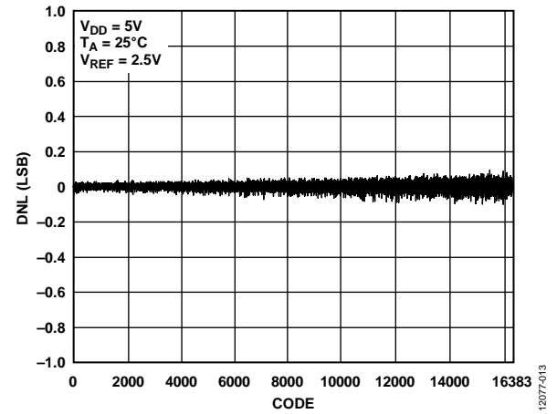
Figure 13. AD5692R DNL
