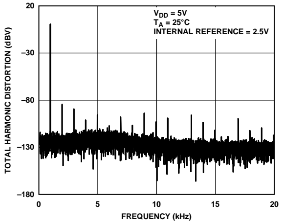
Figure 40. Total Harmonic Distortion at 1 kHz
