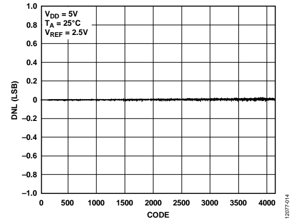
Figure 14. AD5691R DNL
