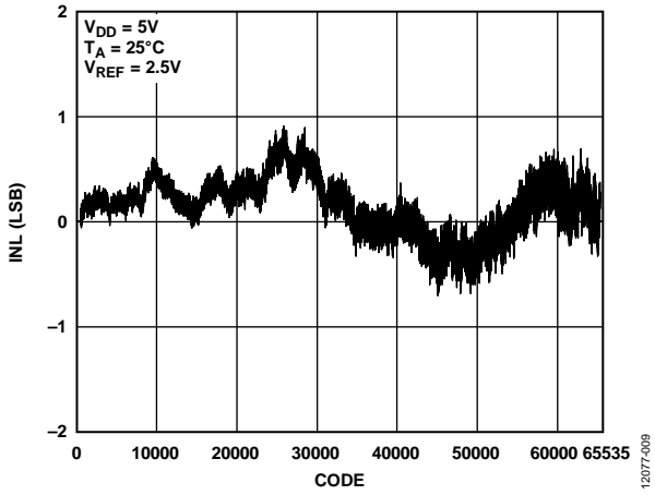
Figure 9. AD5693R/AD5693 INL
