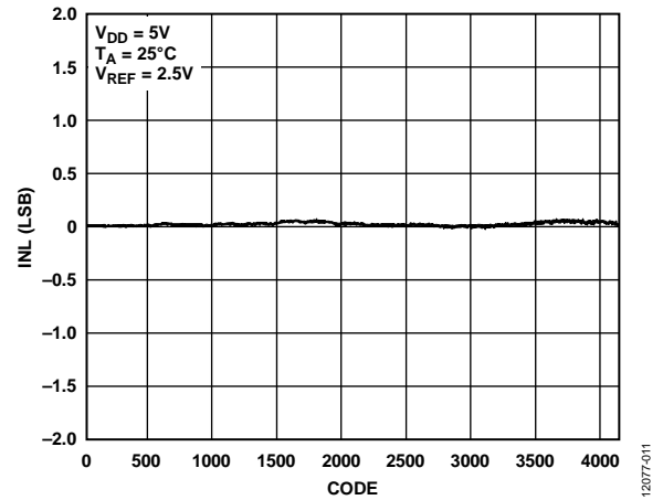
Figure 11. AD5691R INL
