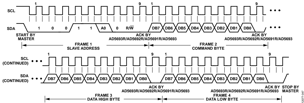
Figure 47. I 2 C Write Operation
