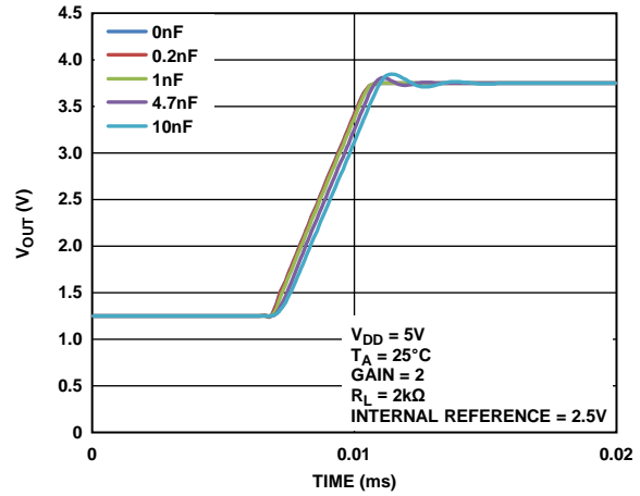
Figure 42. Capacitive Load vs. Settling Time, Gain = 2
