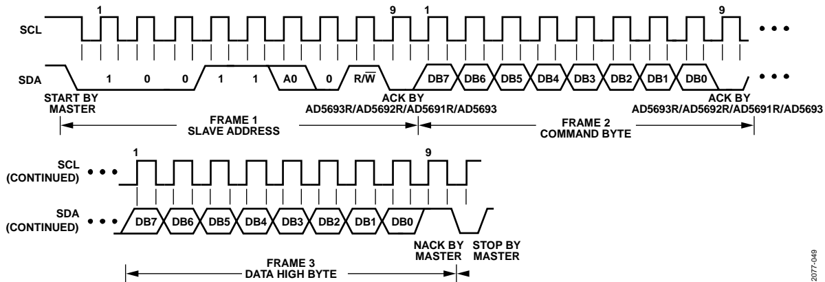
Figure 49. I 2 C Read Operation
