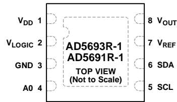
Figure 7. AD5693R-1/AD5691R-1 Pin Configuration, 8-Lead LFCSP, V LOGIC Option
