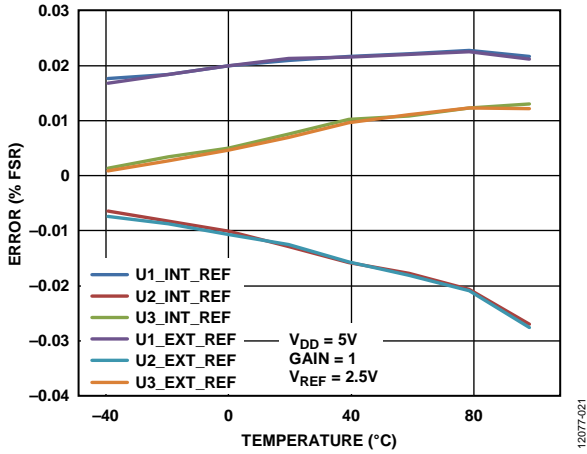
Figure 21. Gain Error and Full-Scale Error vs. Temperature
