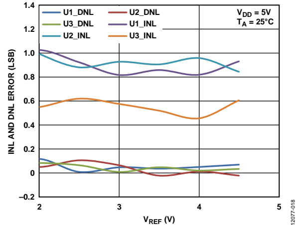
Figure 18. INL and DNL Error vs. V_{REF} (AD5693R/AD5693)
