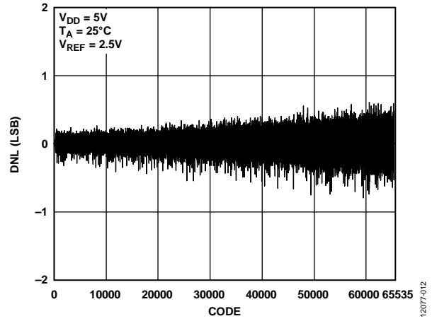
Figure 12. AD5693R/AD5693 DNL
